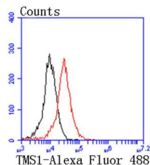
Fig. 2. Flow cytometric analysis of 293 cells with TMS1 antibody at 1/50 dilution (red) compared with an unlabelled control (cells without incubation with primary antibody; black). Alexa Fluor 488-conjugated goat anti rabbit IgG was used as the secondary antibody.
